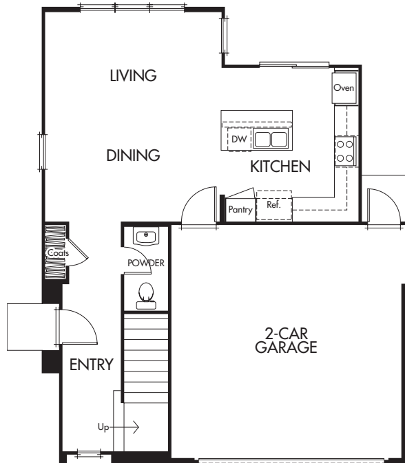
First Floor Walls, windows, doors, decks and porches vary per elevation.
